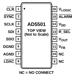
Figure 5. Pin Configuration
