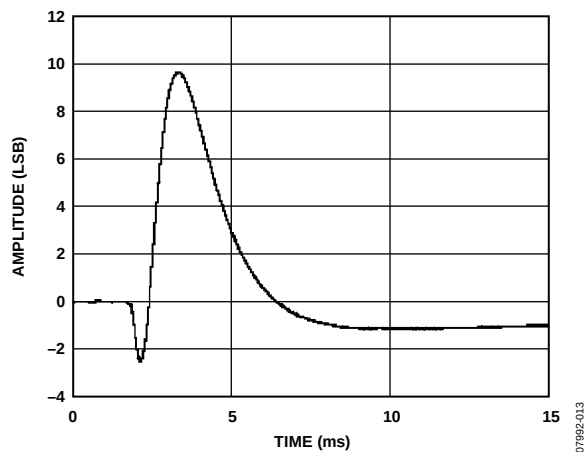
Figure 13. Digital-to-Analog Positive Glitch Impulse
