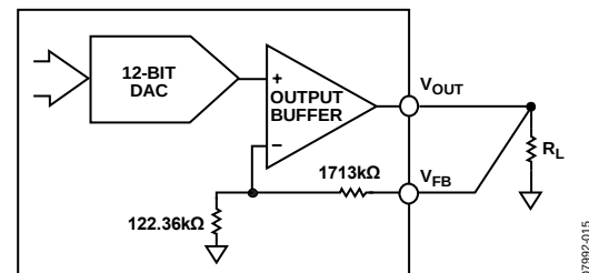
Figure 15. V_{FB} and V_{OUT} Configuration
