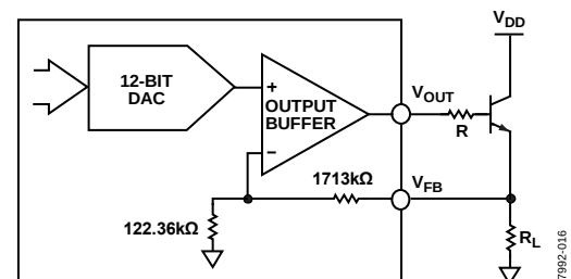
Figure 16. Pass Transistor Configuration
