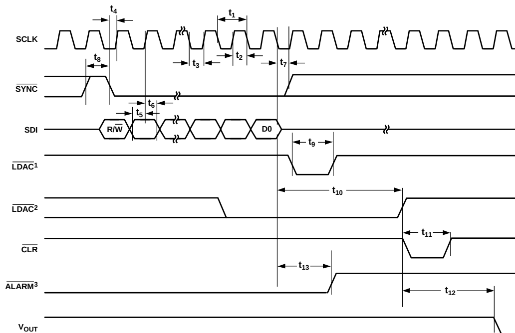
Figure 3. Write Timing Diagram
