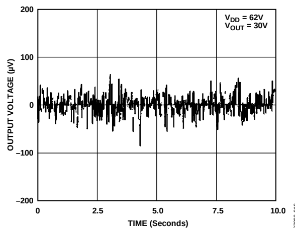
Figure 10. Output Noise
